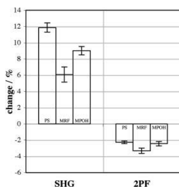
FIGURE 11 Signal changes for 0 mV \rightarrow -50 mV for 910 nm excitation of SHG and 2PF from di-4-ANEPPS, di-4-ANEMRF, and di-4-ANEMPOH. 2PF was collected for wavelengths between 490 nm and 560 nm.
